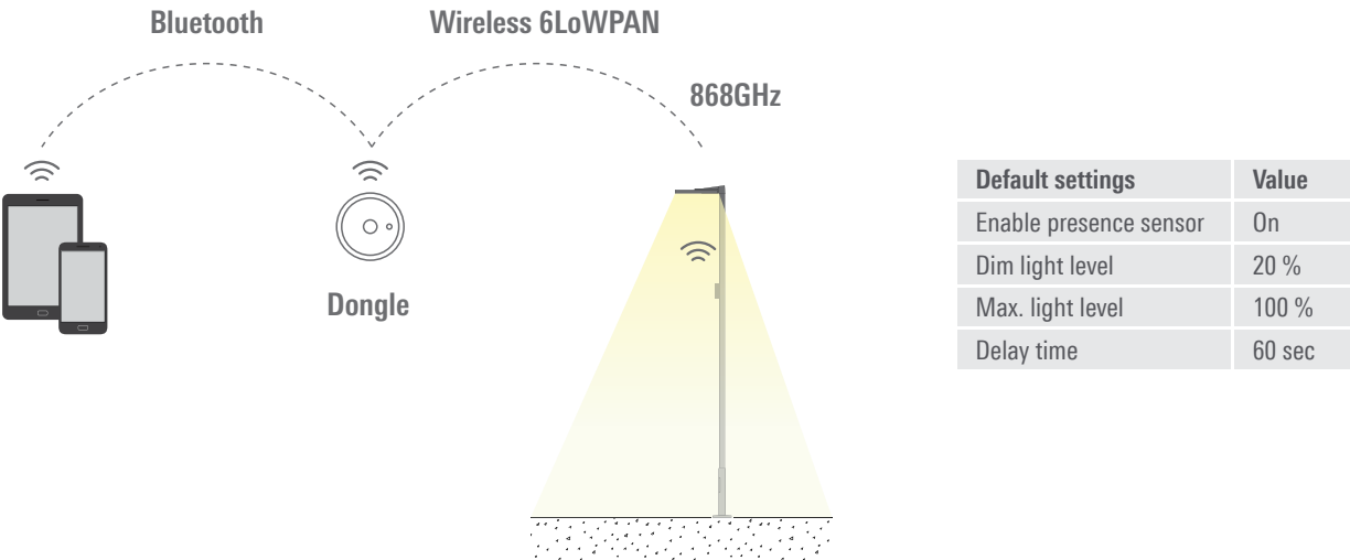
Communication method for commissioning and installation
