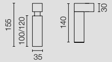
LED ARRAY 6W
