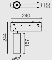
LED ARRAY 25,5W
