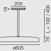
TOP LED 40W
