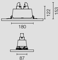
POWER LED 2X6W
