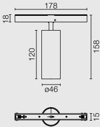
POWER LED 12W
