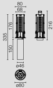
POWER LED 10,5W
