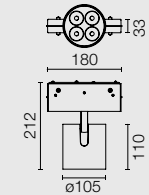
POWER LED 13W
