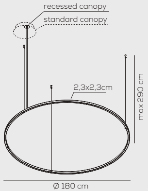
rosone standard /standard canopy
