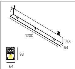
L 1200mm
