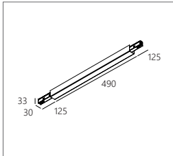
SLM26L - Mid Powerbox 48V/10W
