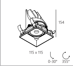
SQUARE KIT
