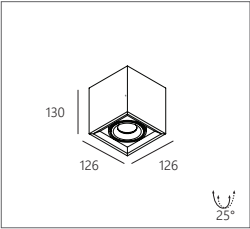
SQUARE (1 HEAD)
