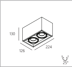
SQUARE (2 HEADS)
