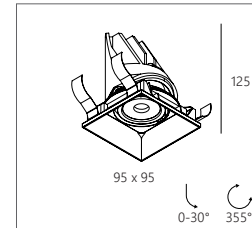
SQUARE KIT
