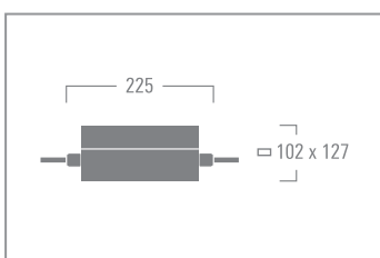
Gear box for DOC240-GB
