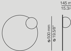
CIR_3702 LED 10W (2700K) Typ* 870 lumens Dimmable triac *Optional dimming available
