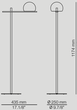
CIR_3728 LED 8W (2700K) Typ* 665 lumens On/Off cord switch *Optional dimmer available
