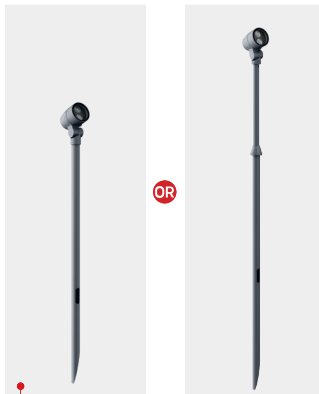
AUN-POL-0188-XX Cylindrical aluminium pole, diameter 105mm, H= 522mm
