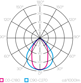
light distribution DOWN MPRM
