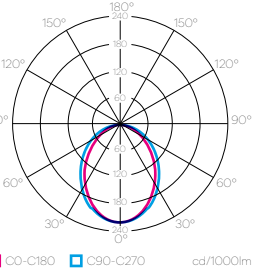
light distribution DOWN OPAL
