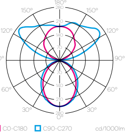
light distribution UP & DOWN OPAL
