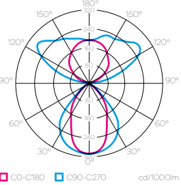
light distribution UP & DOWN MPRM
