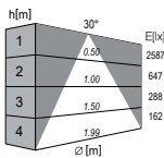
FreePlus Tunable White CR193, 3000K 30°
