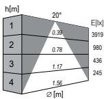
FreePlus Tunable White CR193, 3000K 20°
