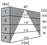
FreePlus Tunable White CR193, 3000K 40°
